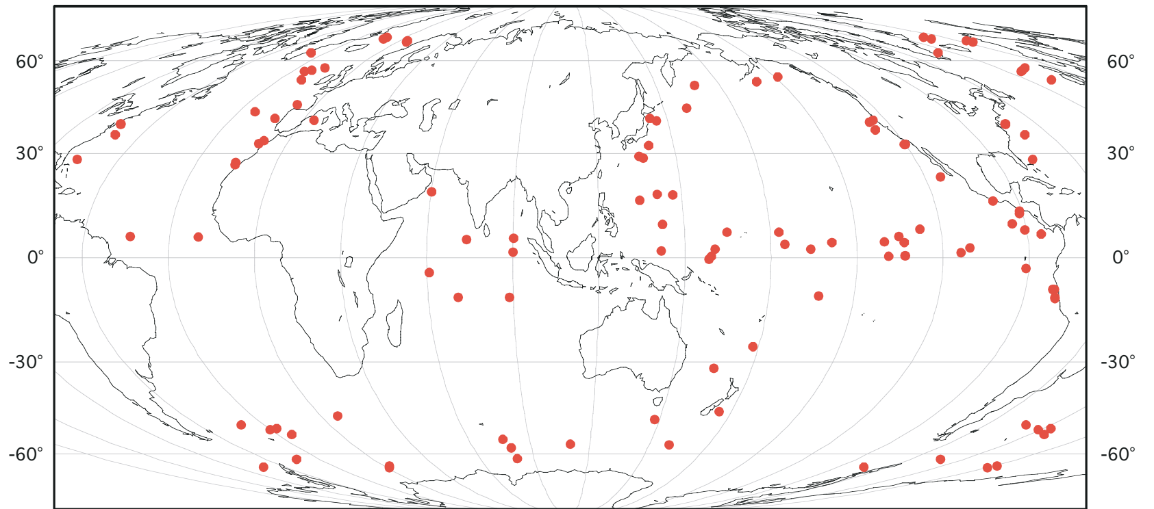
Mid Miocene Rad MRC Samples
